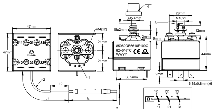
1. Sealing; 2. Sleeve; 3. Manual reset button; 4. Plastic cap(Black)
